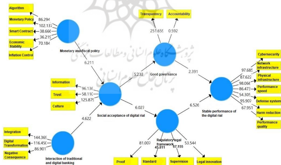
Figure 4. T-Values
