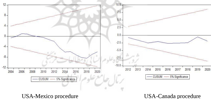
Figure 3. CUSUM results for scenario 2. USA trade deficit
