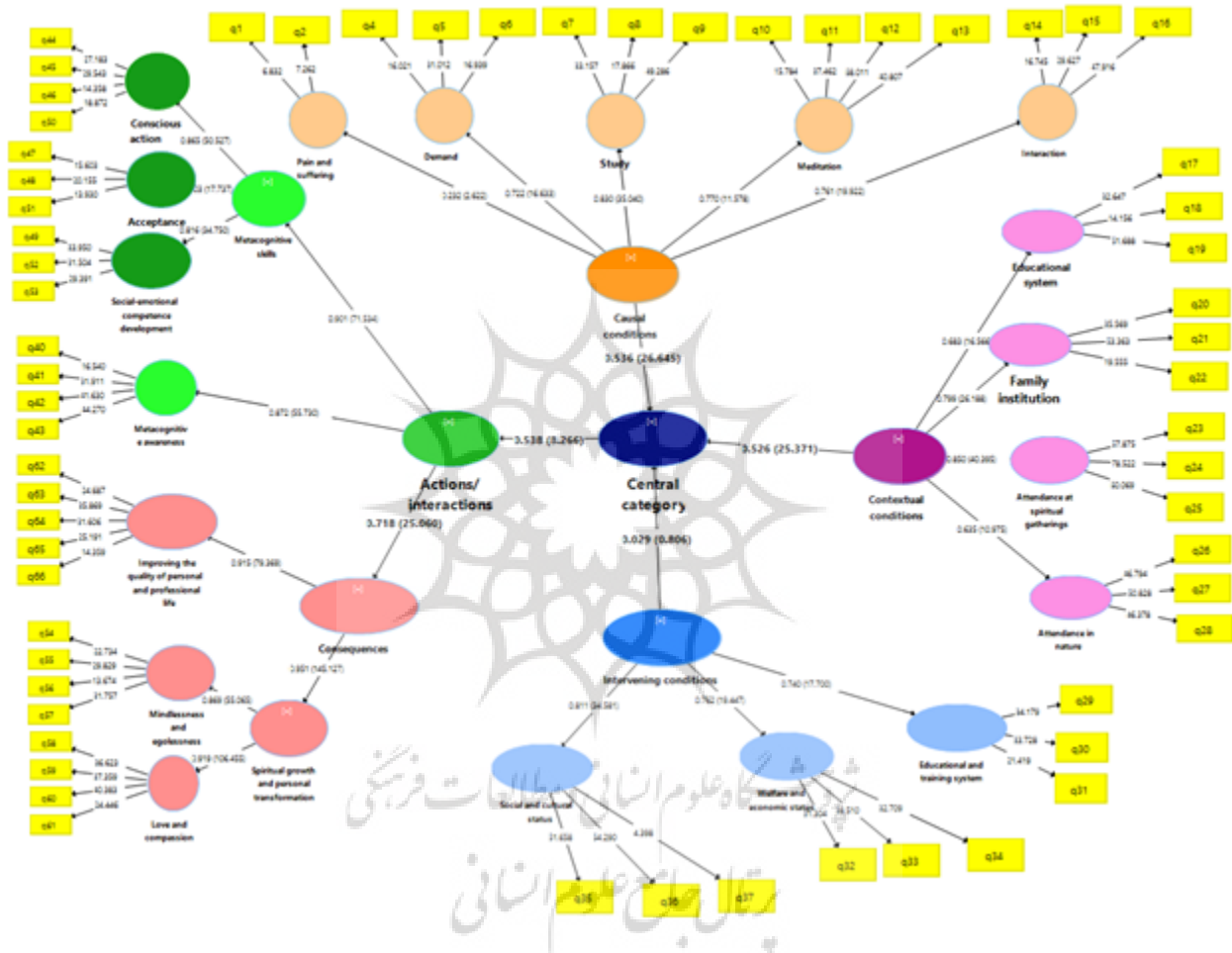
Figure 3: Structural Model Showing Beta Coefficient and t-Statistic
