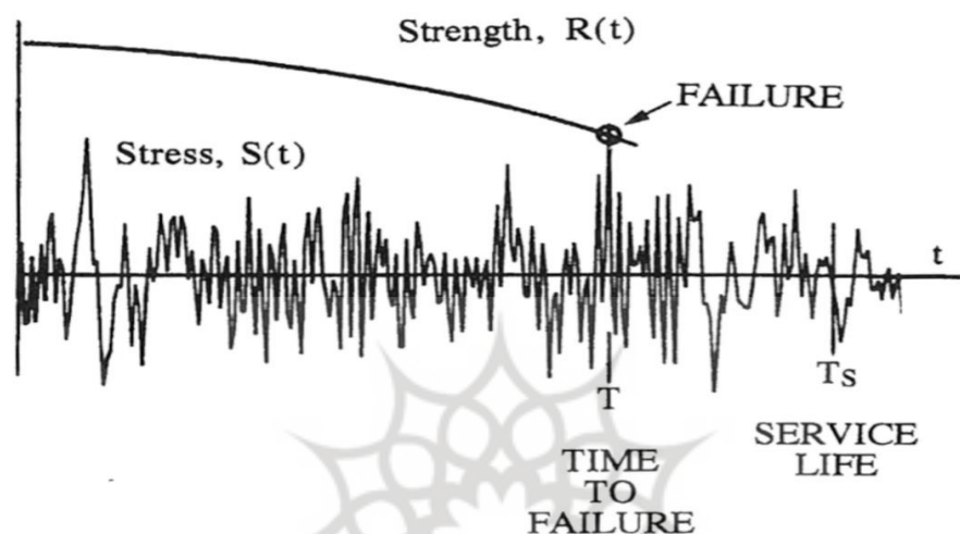
Figure 5. The first-passage failure
