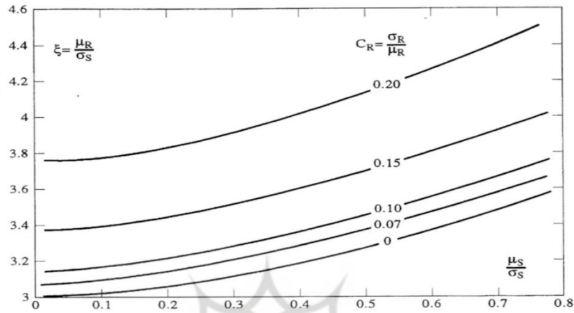
Figure 3. The graph for C_R with different values of \zeta
