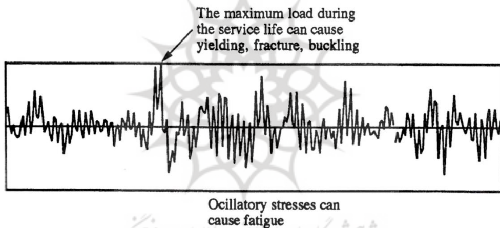
Figure 1. The state of stress on an element over time
