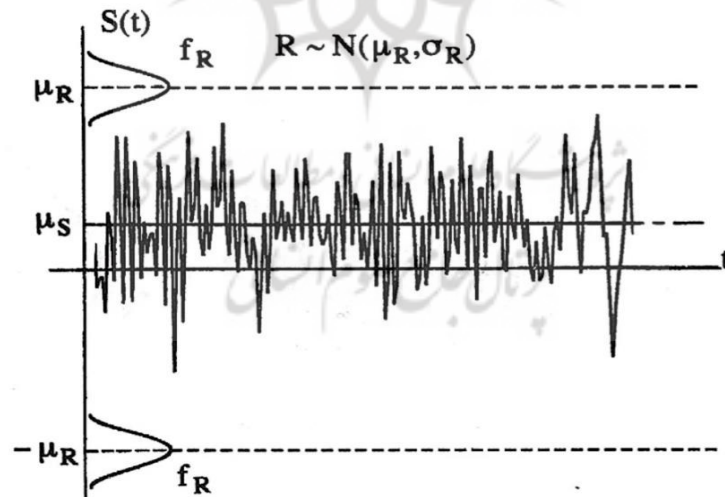
Figure 4. Stationary stress process S(t) with a non-zero mean and random strength R
