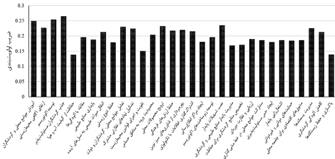
RReliefF
