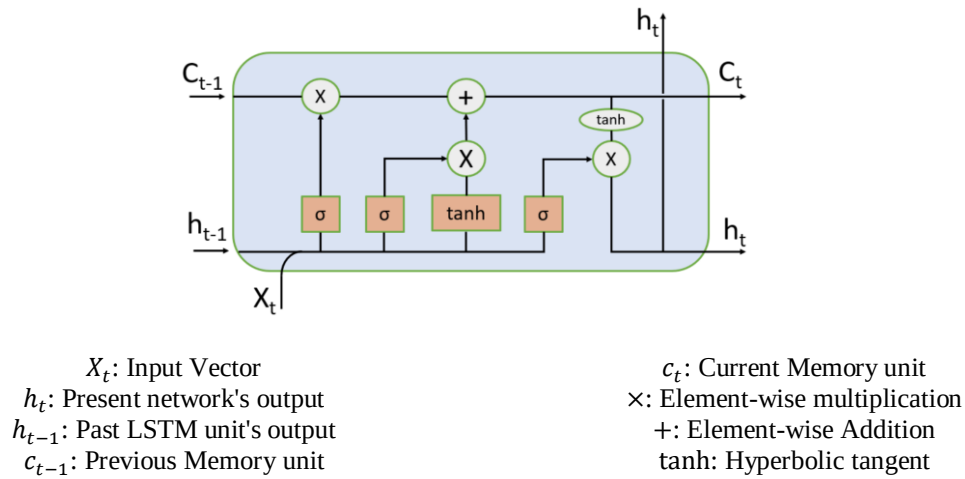
Figure. 2-Long Short-Term Memory (LSTM) neural network
