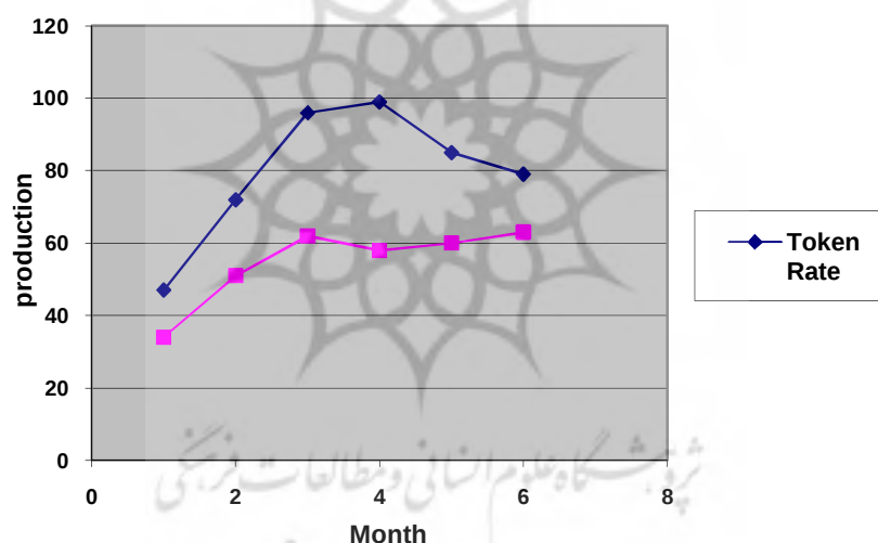
Figure 4. Type/token growth
