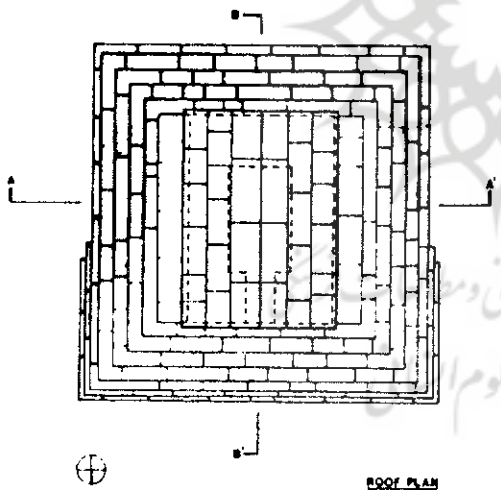
ROOF PLAN
