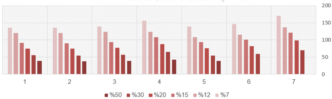
Fig. 2: Comparison between single-glazed glass in heating
