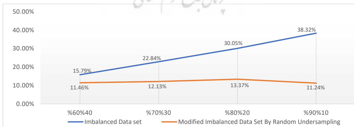
Fig 10: Comparison of type I error of SVM based on modified imbalanced and imbalanced data
