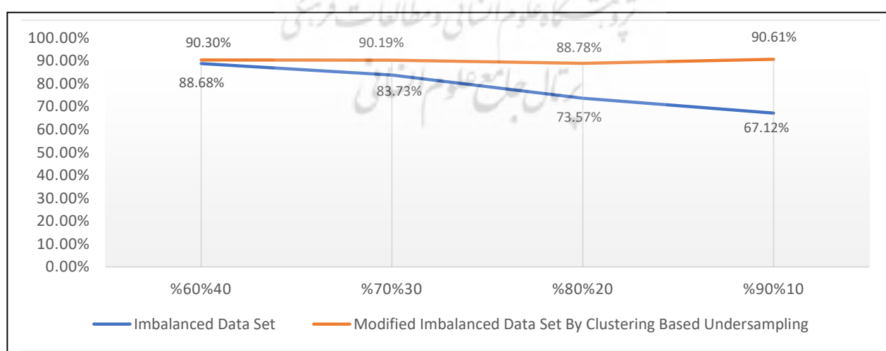
Fig 21: Comparing geometric mean in Random Forest based on modified and imbalanced data
