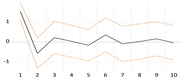
Response of R to R long-run
