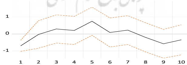
Response of R to Shock EU long-run
