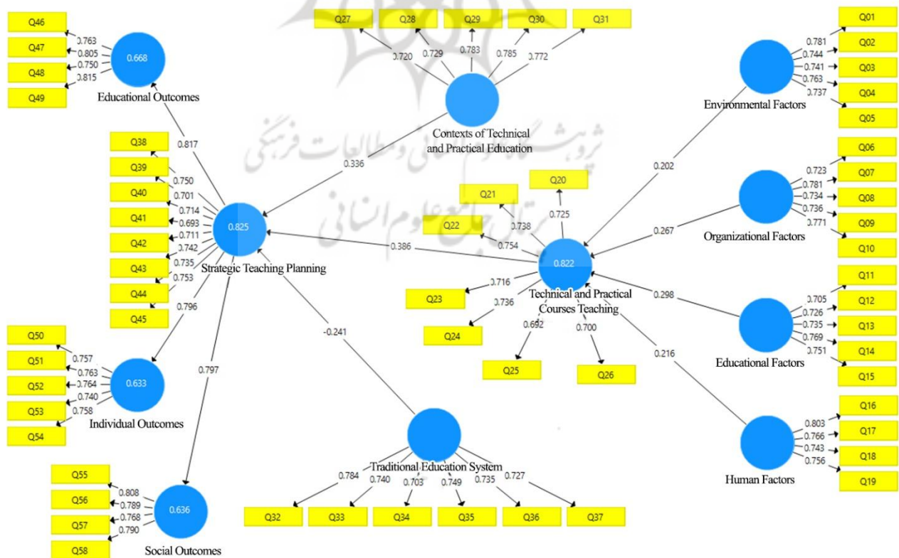
Model Validation Output using Partial Least Squares (Standard Coefficients)
