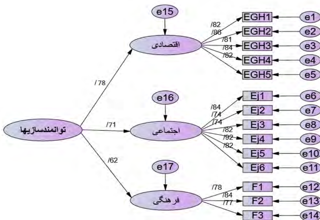
Diagram2: Second-order confirmatory factor analysis model of enablers
