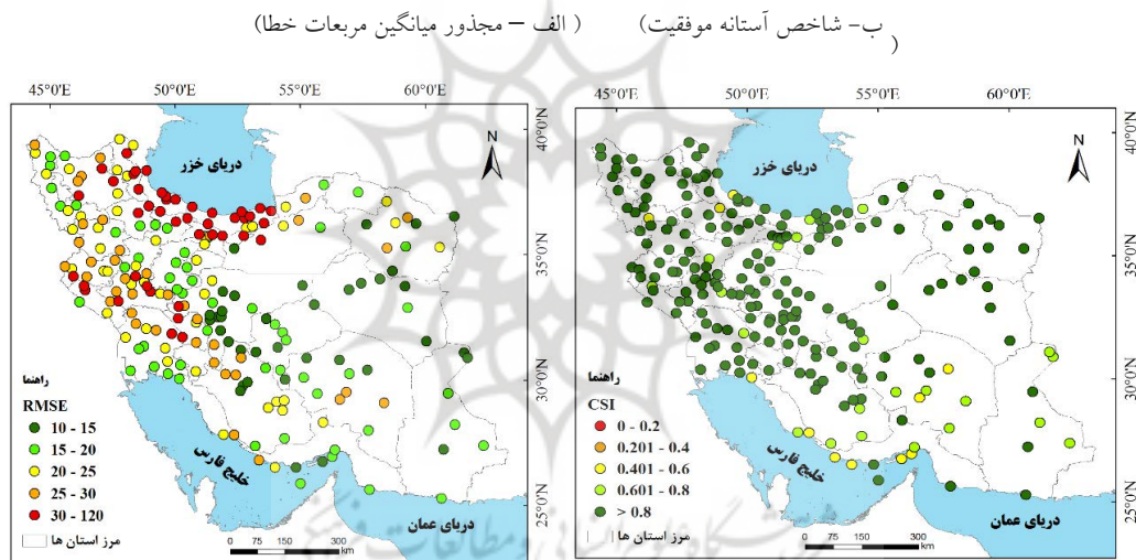
Figure 5. Evaluation of the efficacy of MERRA satellite-derived precipitation products utilizing assessment metrics
