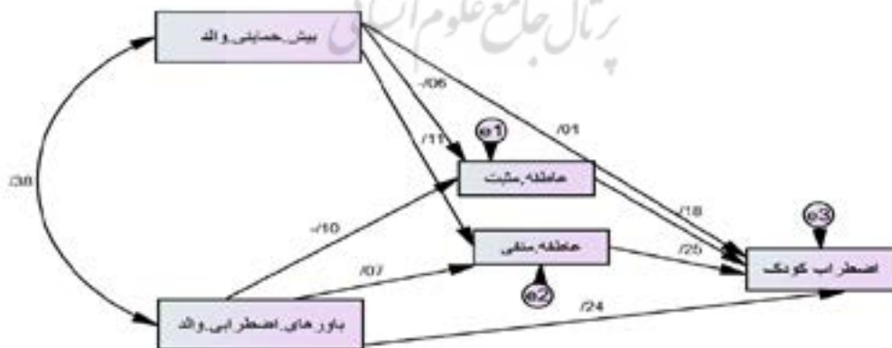
Figure 1. Standard coefficients of the final model
