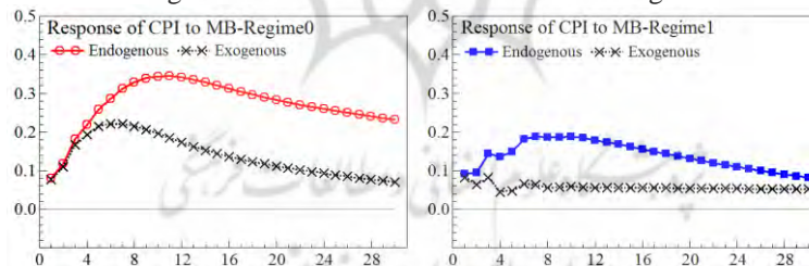
Chart 3: The IRF of Prices Level to Monetary Impulse in Endogenous and Exogenous Models devided Zero and One Regimes
