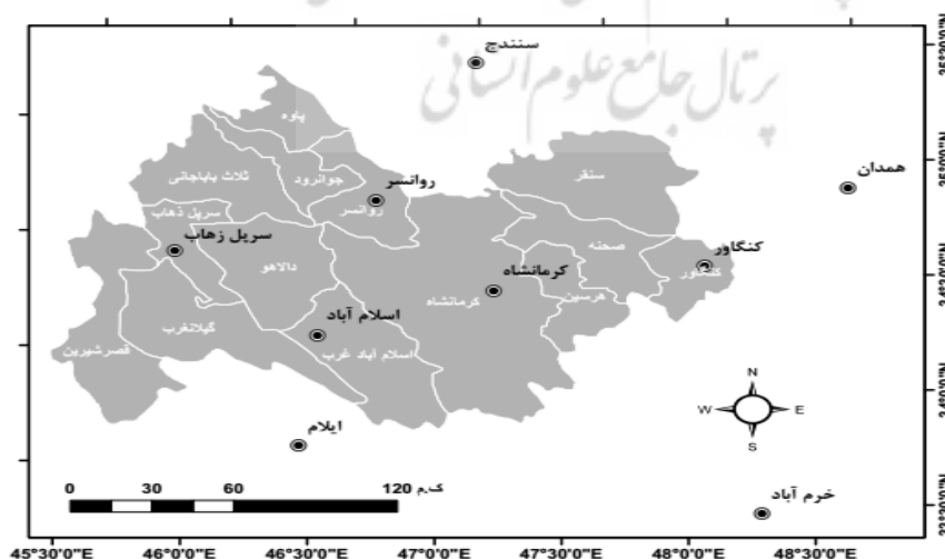
▲ Figure 1. Location and distribution of the studied synoptic stations
