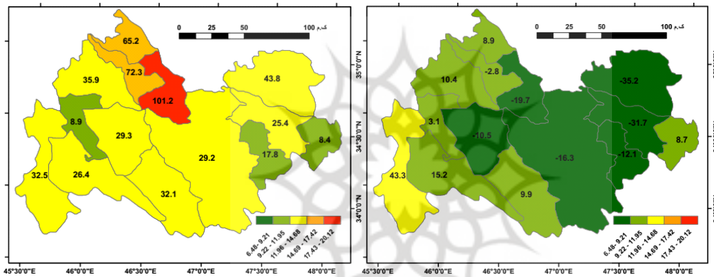
▲ Figure 5. Left (scores) color (the criterion of phenomena), the figures on the map are the percentages of change in the first interval compared to the base interval. Right: scores and percentages of change in the second interval compared to the base interval
