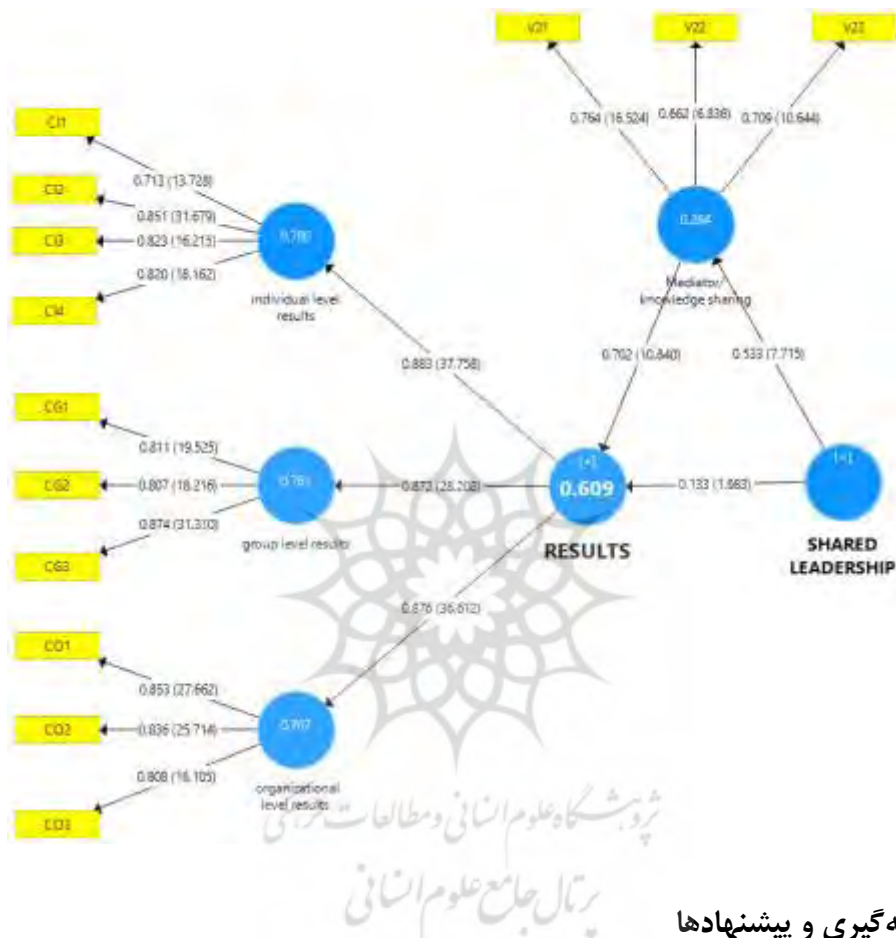
Figure 2: Path coefficients and significance values of the structural model of the research
