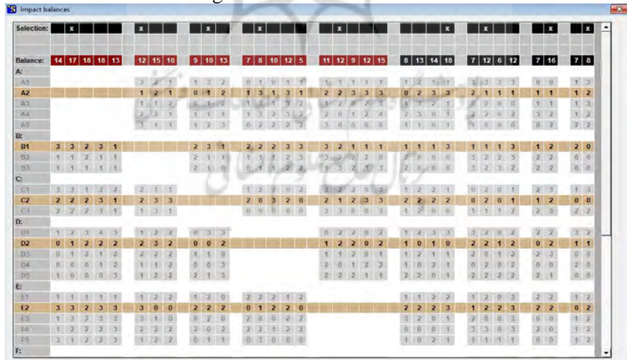
Figure.3: Cross-matrix homogenization
