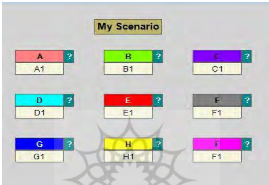
Figure.4: Identified scenarios
