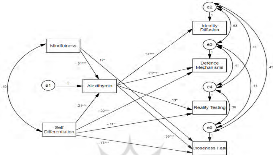
Fig 2. Mediation model.
