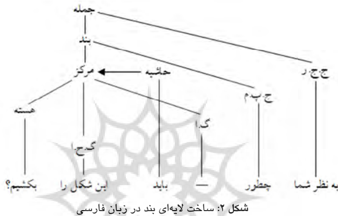
Figure 2: The layered structure of clause in Persian
