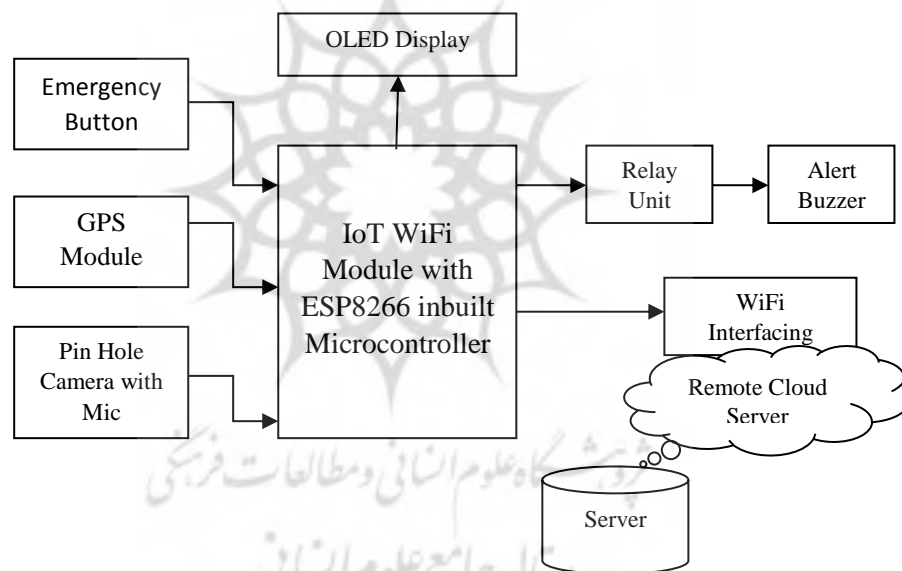
Figure 3. Transmitter Section
