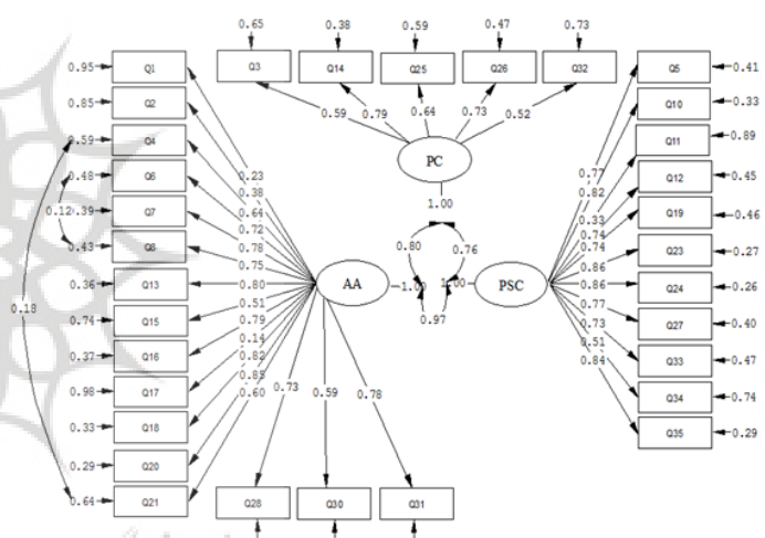
Chi-Square=1174.79, df=459, P-value=0.00000, RMSEA=0.081
