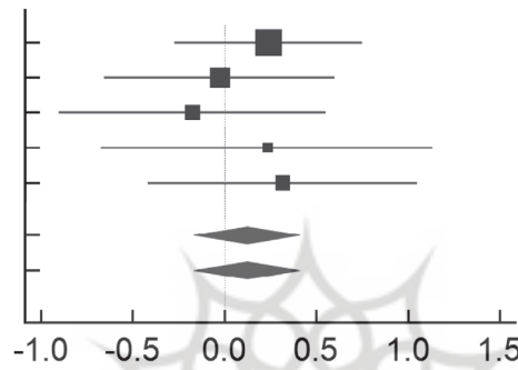
Standardized Mean Difference
