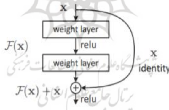
Figure 12. Building block of ResNet
