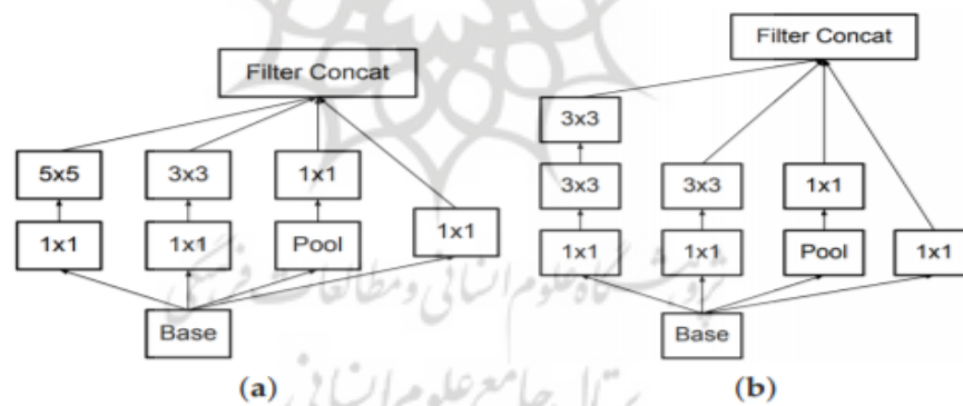
Figure 11. (a) Inception module of GoogLeNet; (b) Inception-v2 module
