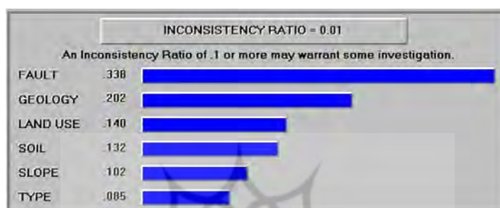
Figure 3. Two-by-two comparison of different parameters in creating an earthquake
