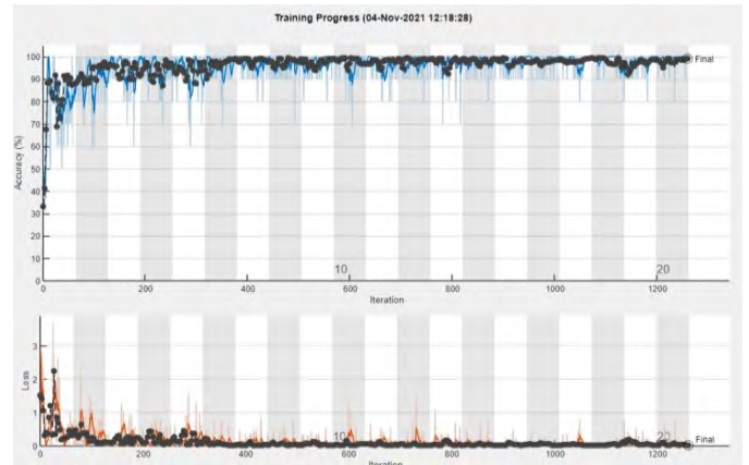
Figure 3. Training Process
