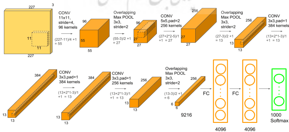
Figure 1. Alexnet Architecture
