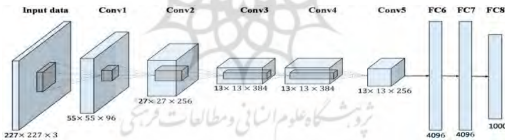
Figure 1. Alexnet Architecture
