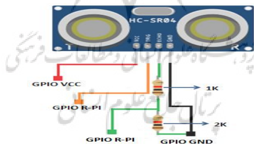
Figure 3. Potential divider circuit for HC-SR04.
