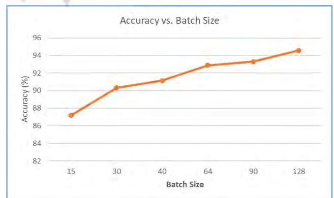
Fig. 7. CoReHAR Accuracy vs. Batch Size
