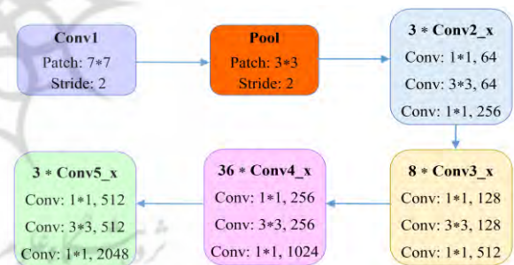
Fig. 1. The basic architecture of ResNet152
