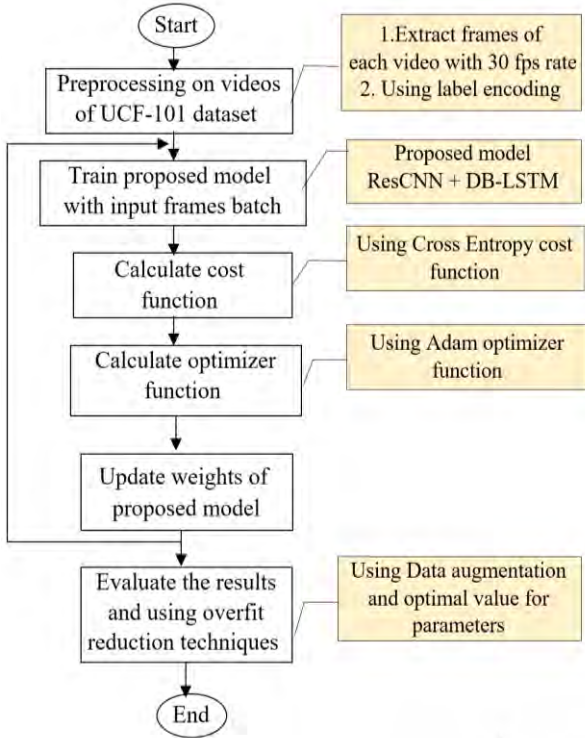
Fig. 5. Flowchart of proposed model
