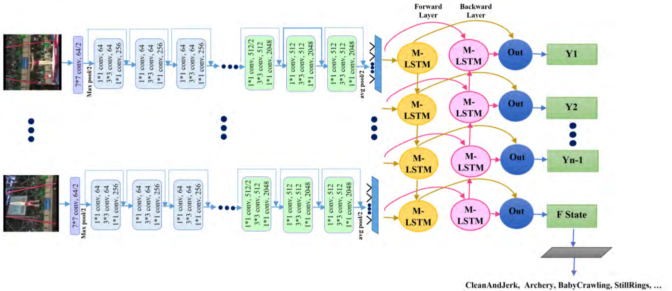
Fig. 3. Detailed structure of the proposed CoReHAR method
