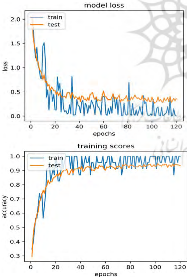
Fig. 6. Accuracy and loss diagrams of the proposed model in both training and testing steps
