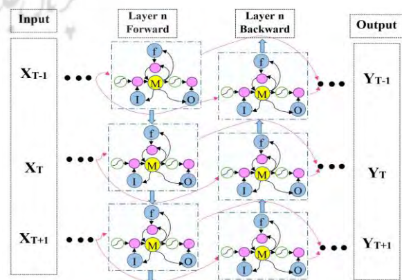
Fig. 2. The basic architecture of DB-LSTM
