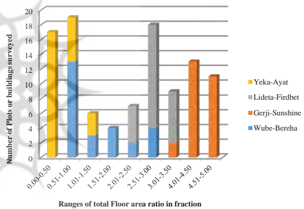
Fig. 12: Total Floor area Ratio in four cas study Settlements in Fraction
