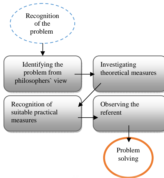
Fig.1: Research model
