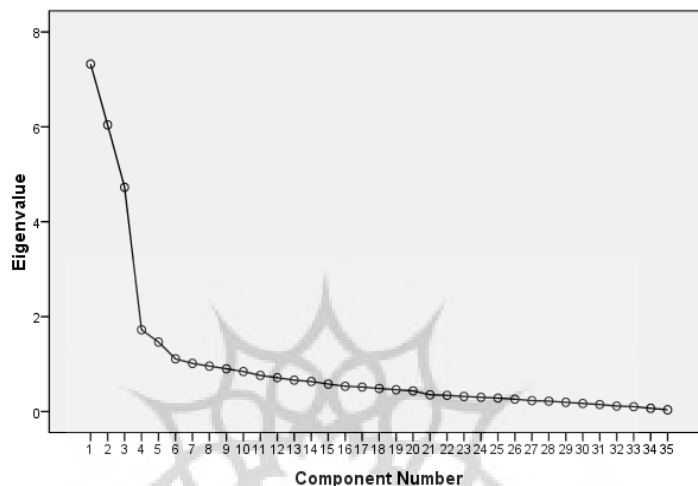
Scree Plot
