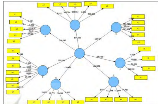
Figure 7. Factor Loadings
