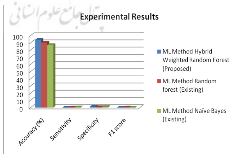
Figure 2. Experimental results Graph for Naïve Bayes (De Caigny, et al., 2018), Random Forest(Akbarabadi, M., & Hosseini, M. 2020), and Proposed HWRF Method
