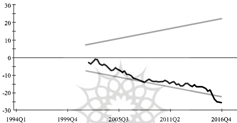
Figure 2. The Result of the CUSUM Test.
