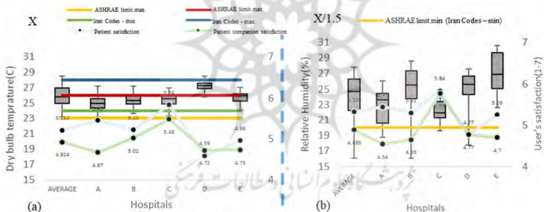
Fig. 1. Dry bulb temperature (a) & Relative humidity (b) range in hospitals
