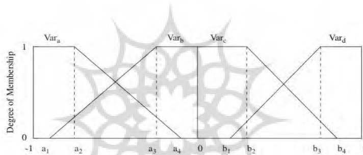
Fig. 3: Trapezoidal Membership Function for the Input Linguistic Variables
