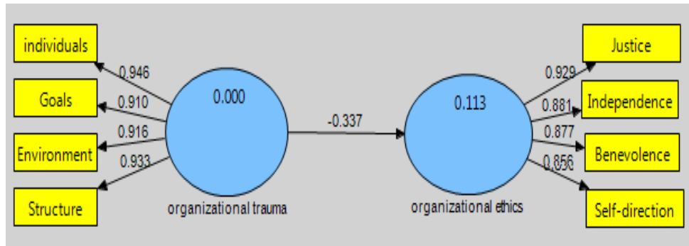
Fig 3. The research model and standardized factor loading coefficients
