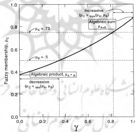
Fig.3; A graph of fuzzy membership, \mu_c , obtained by combining two fuzzy memberships, \mu_A , and \mu_B . (Graeme f. Bonham-carter, 2006).
