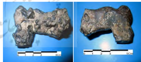
Fig10. Right: Upper Surface of the Specimen with Bulging, Reform Morphology that Reflects Plastic Deformations of the Melt during its Freezing Process; Left: Lower Surface of the Specimen Characterized by Relatively Irregular Morphology, Concentration of Secondary White Minerals Around
