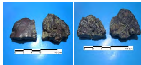
Fig8. Right: Upper Surface of the Flat Slags with Flow Wrinkles; Left: Lower Surface of the Specimen with Flat Morphology at the Left in Contrast to Irregular Morphology of Upper Surface at the Right.
