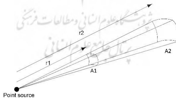
Fig. 4-3: Total energy passes from A1 to A2 uniform, whereas A is proportion to r^2 , then energy density or intensity is proportion inversely to r^2 .
