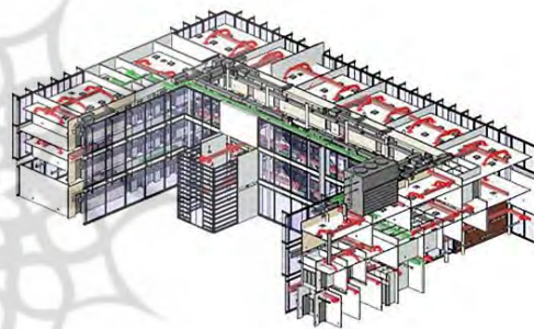
Fig. 3 Mechanical, electrical and plumbing (MEP) modelling (Autodesk, 2018)
