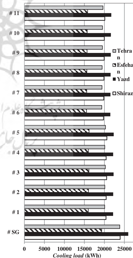
Fig. 16 Total annual cooling load of office building, Tehran, Esfahan, Yazd and Shiraz
