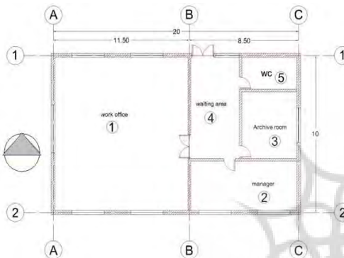
Fig. 7 Plan of office building for simulation
