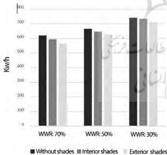
Fig. 7 Heating load for the interior spaces during a year
