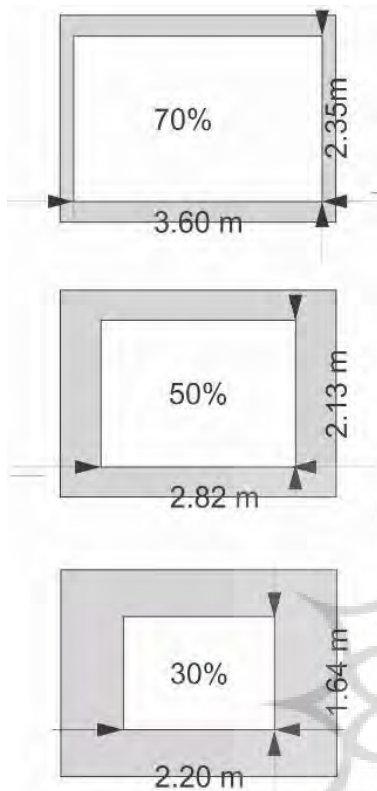
Fig. 4 Different window to wall ratios (WWR)
