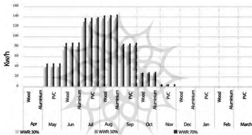
Fig. 17 Monthly cooling load for the interior spaces
