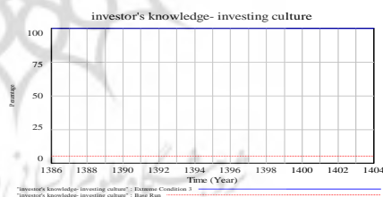
investor's knowledge-investing culture investor's knowledge-investing culture : Extreme Condition 1 investor's knowledge-investing culture : Base Run
