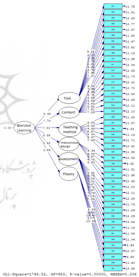
Figure 2. T-value Statistic of Independent Variables
