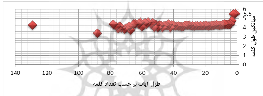
Diagram 3: Relationship between Verses' Length and Word's Length
