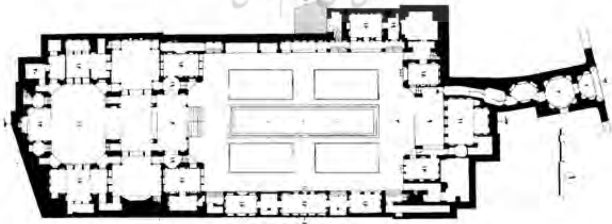
Fig.3 – The first floor plan of Borojerdies' house
