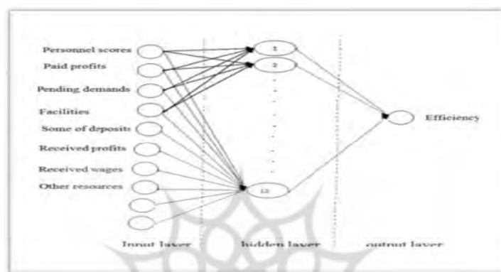
Figure 1: Topology of the Proposed Network
