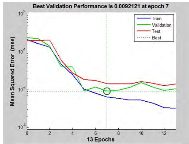
Figure 2: Error in the training, validation and test process
