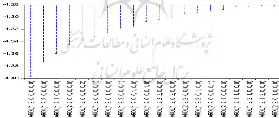
Schwarz Criteria (top 20 models)
